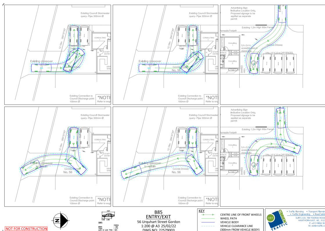
Figure 3: Swept paths after reduction in car parking
