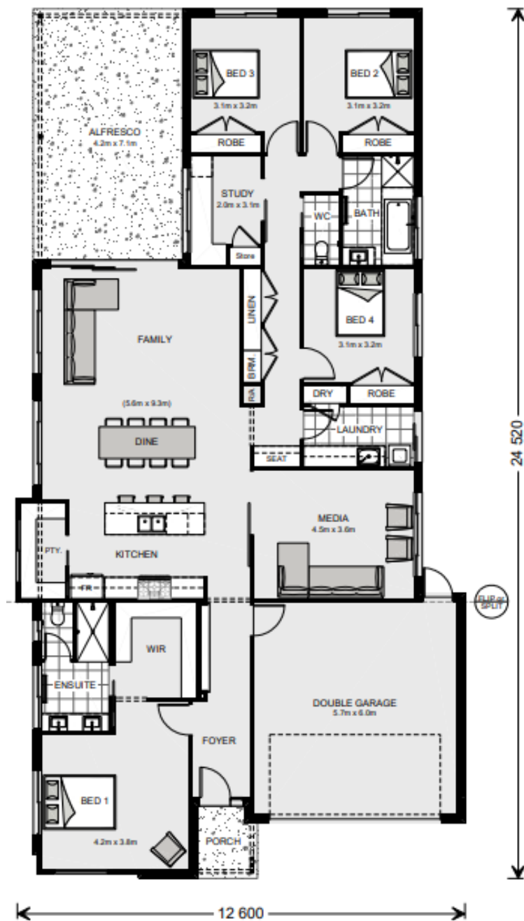
Figure 4: Floor plan of the dwelling
