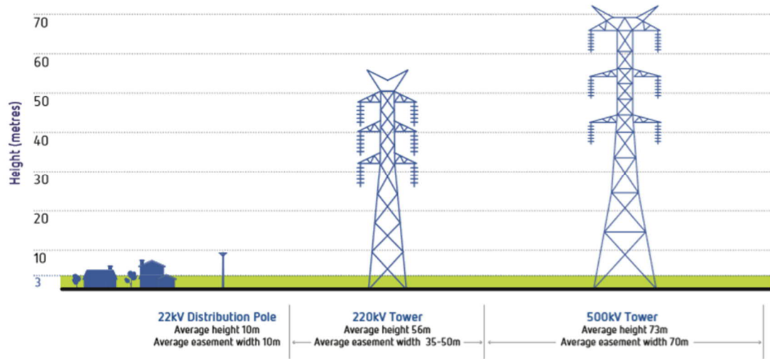
Figure 1: Average tower height and easement widths
